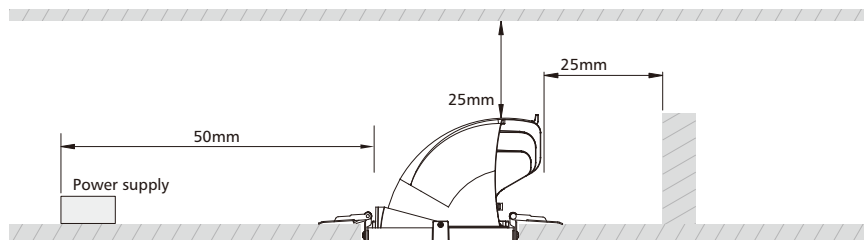
Encastrement / Ceiling cutout table
