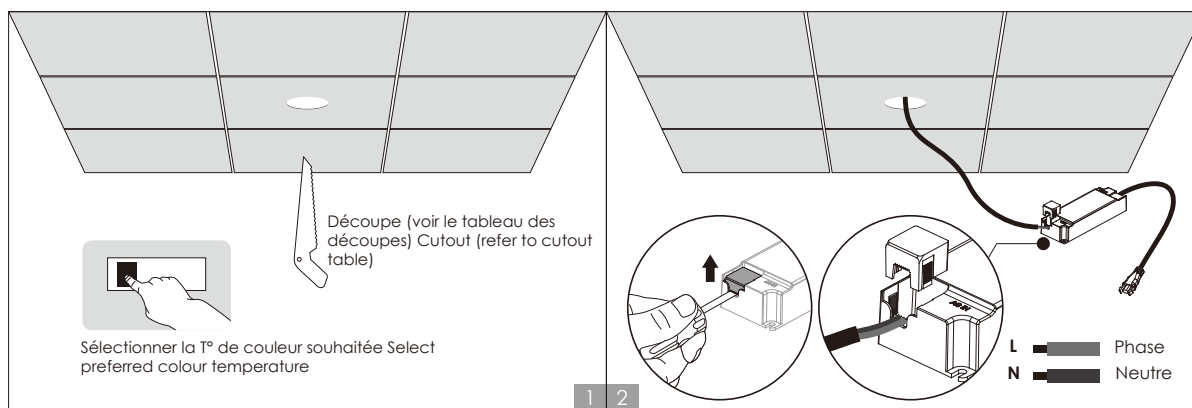
Fig 2: Installation
